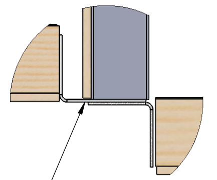
MIDDLE SIZE BRACKET INSIDE, SMALL BRACKET OUTSIDE, IN ORIENTATION SHOWN DETAIL G
